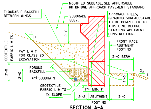
SECTION A-A BACKFILL DETAILS
