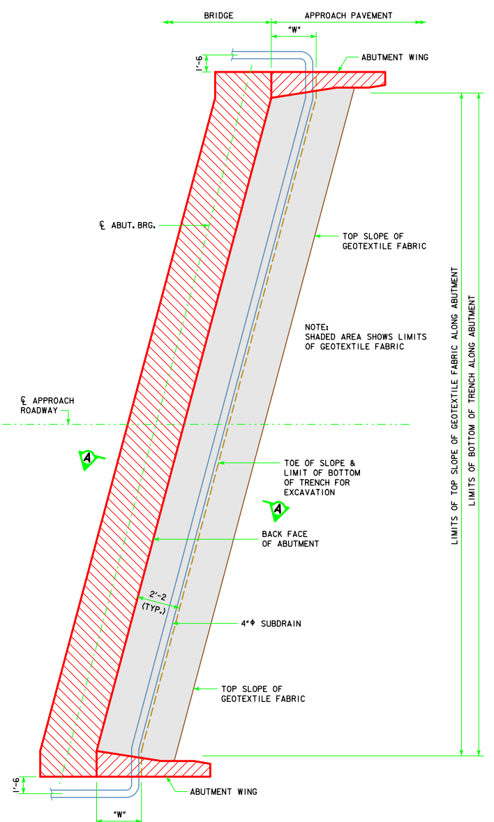
SKEWED ABUTMENT PLAN WITHOUT WING EXTENSIONS (SKEWED LEFT AHEAD SHOWN, SKEWED RIGHT AHEAD SIMILIAR)
