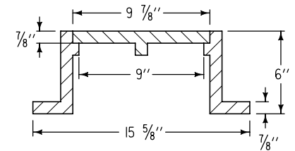
CASTING ① (Dimensions are nominal)
