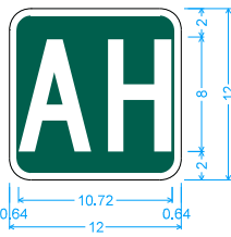
D10-8A: 1.50" Radius, 0.50" Border, White on Green; [AH] C 2K;
