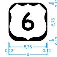
D10-5; 1.50" Radius, No border, White on Black;
