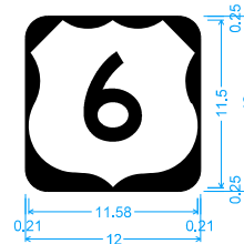
D10-5A: 1.50" Radius, No border, White on Black;
