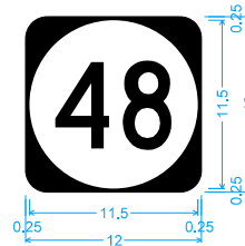
D10-9A: 1.50" Radius, No border, White on Black; Rounded Rectangle 5.75" Radius;
