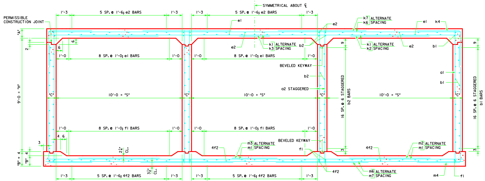
TRIPLE 10 x 9 BARREL SECTION
