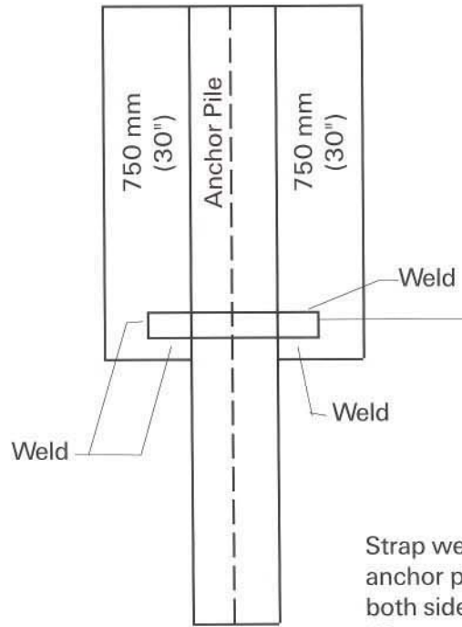
End View No. 1
