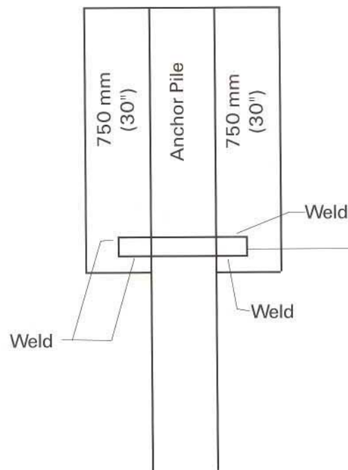
End View No. 2
