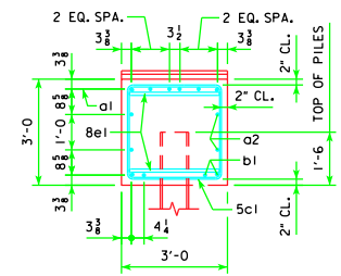
VIEW A-A FOR 11, 12, 13, 14, 15 & 16 PILE BENTS
