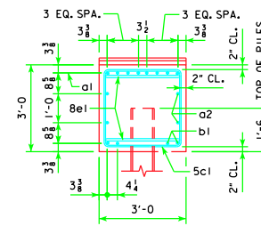
VIEW A-A FOR 9 & 10 PILE BENTS
