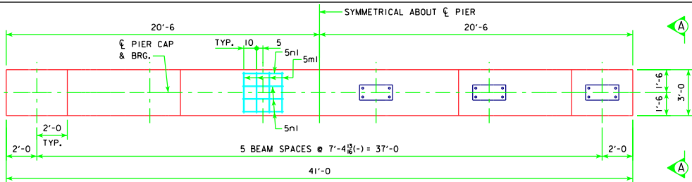
TYPICAL PLAN
