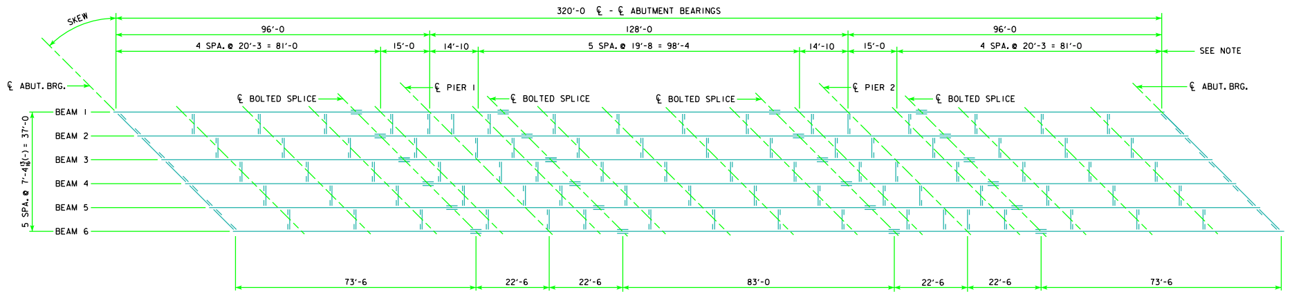
45° SKEWED FRAMING PLAN (R.A. SHOWN, L.A. SIMILAR)
