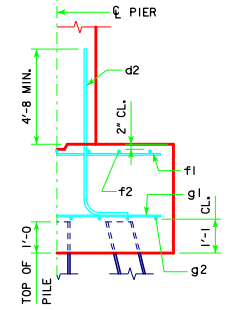
TYPICAL SECTION
