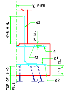
TYPICAL SECTION
