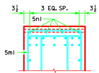
5m1 & 5n1 BAR LAYOUT
