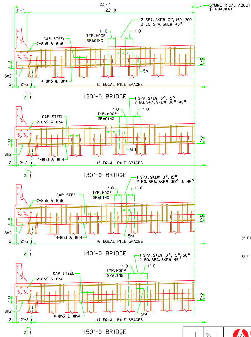
HALF SECTION NEAR PIER SHOWING STIRRUP SPACING AND NUMBER OF PILING NOTE: BOTTOM OF CAP ELEVATIONS WILL BE REQUIRED AT THE CL OF ROADWAY AND AT EACH EXTERIOR PILE.
