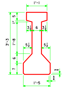
"B" BEAM CROSS SECTION
