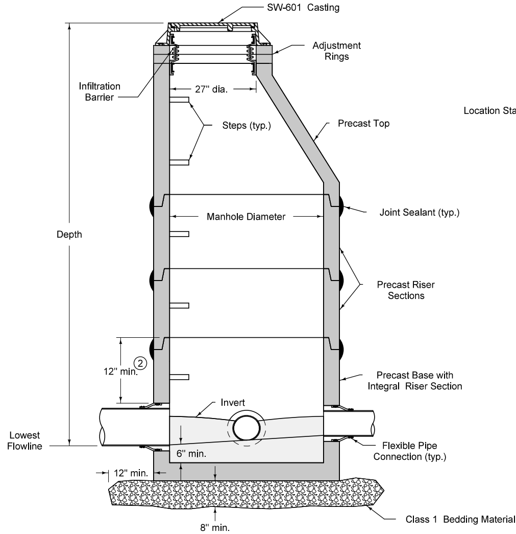
TYPICAL SECTION
