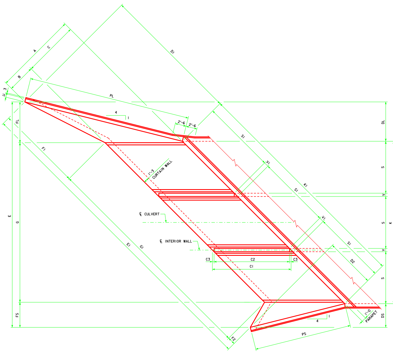
PLAN VIEW
