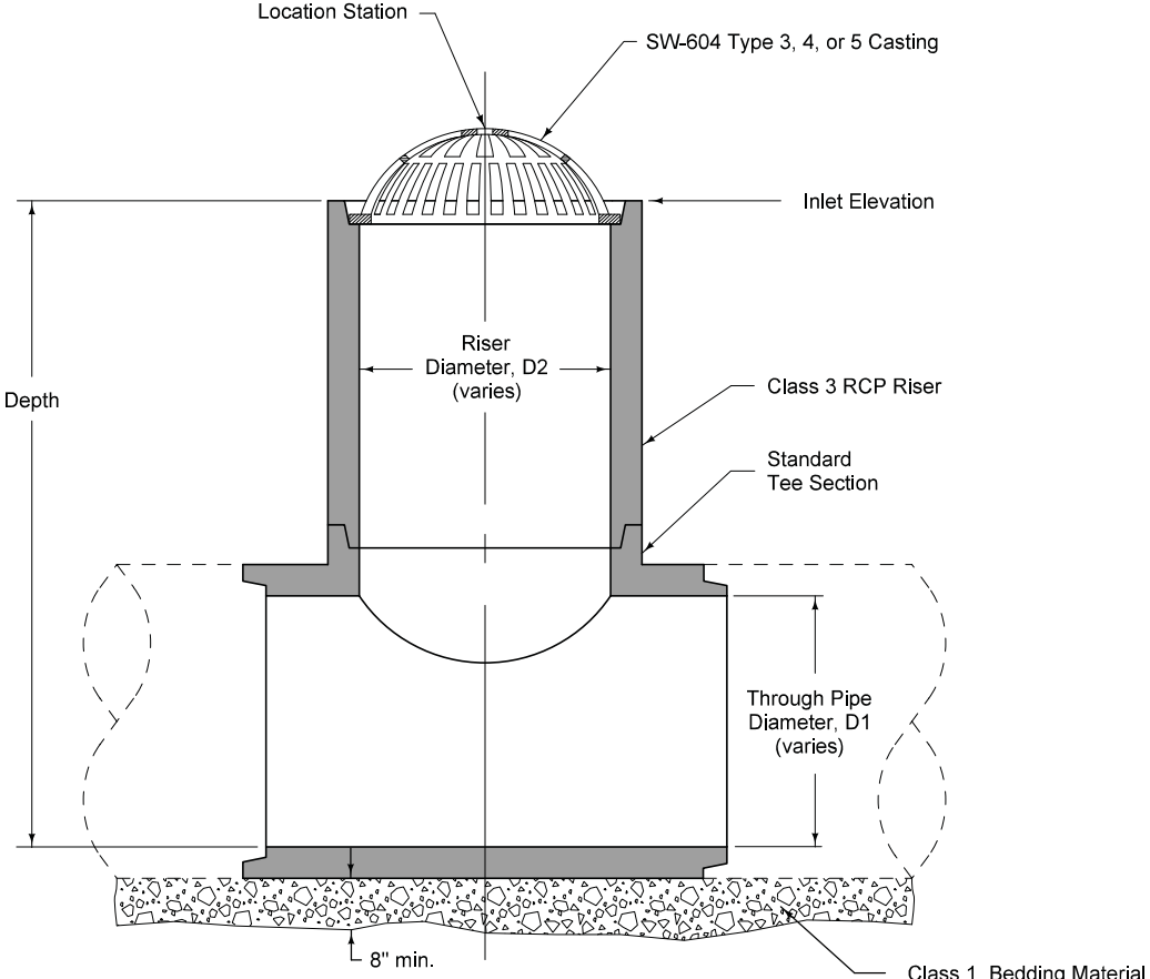
TYPICAL SECTION
