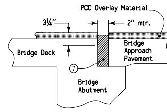
DETAIL 'E'
