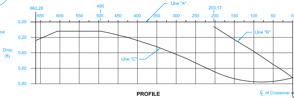
PROFILE
