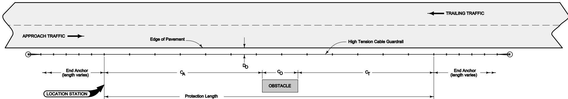
ROADSIDE OBSTACLE, TWO-WAY PROTECTION
