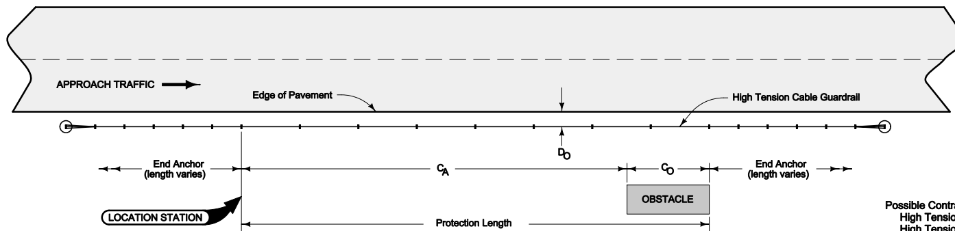
ROADSIDE OBSTACLE, ONE-WAY PROTECTION
