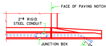
PART PLAN AT WING
