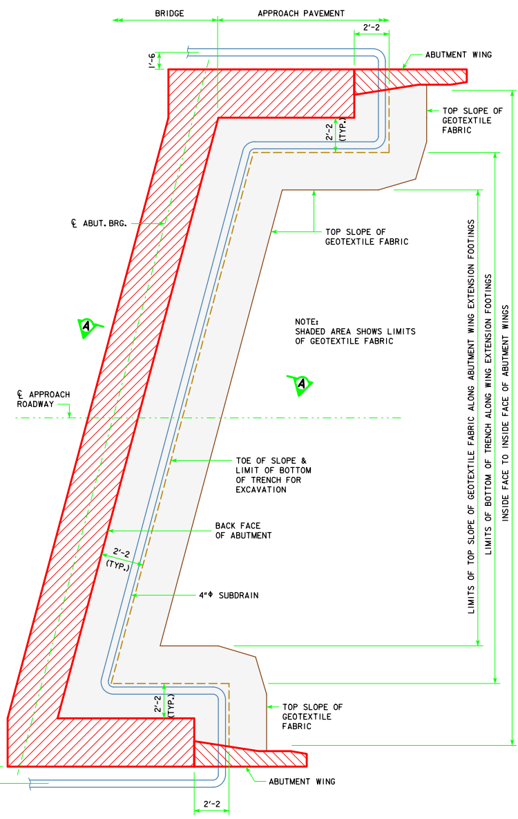
ABUTMENT PLAN WITH WING EXTENSIONS
