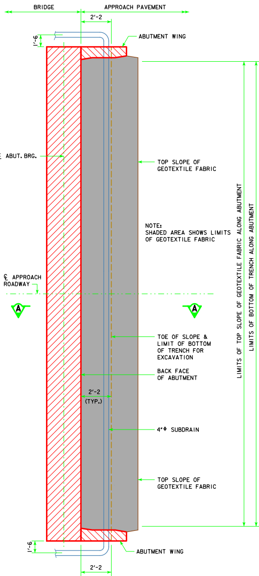
ABUTMENT PLAN
