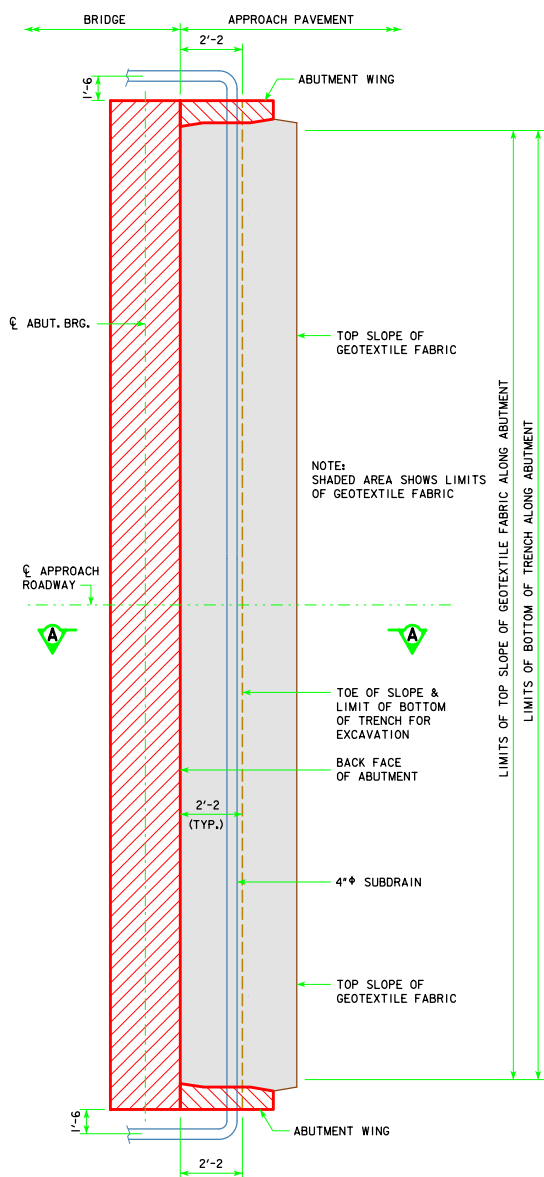
ABUTMENT PLAN
