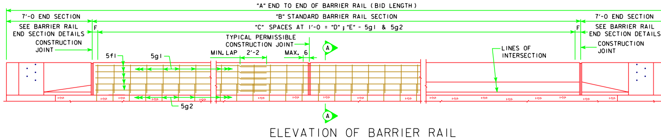
ELEVATION OF BARRIER RAIL
