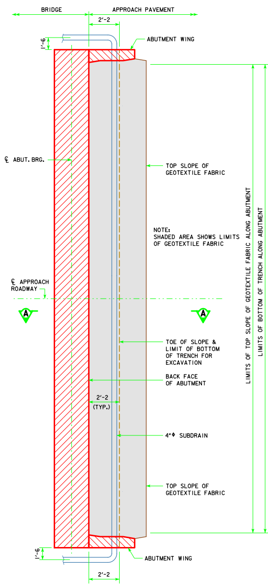
ABUTMENT PLAN
