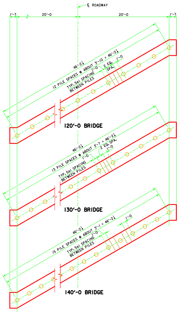
PILE PLAN - 30° SKEW WOOD PILING
