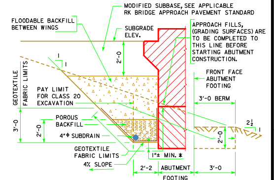
SECTION A-A BACKFILL DETAILS
