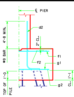
TYPICAL SECTION
