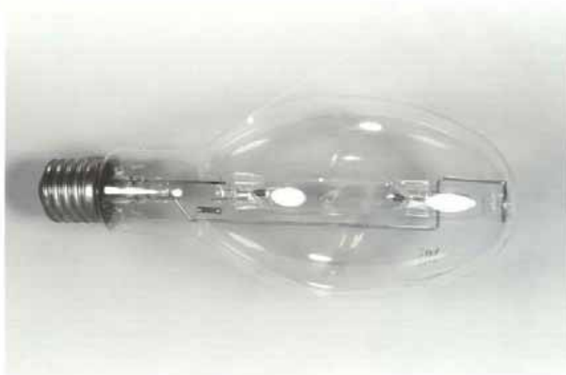
Photograph #5 High Pressure Sodium bulb. These bulbs look about the same as Mercury vapor, but are clear. They are also identifiable by a metal rod which supports the element.
