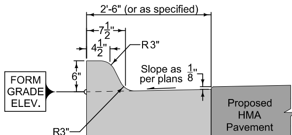
6" STANDARD CURB AND GUTTER
