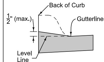
DROP CURB AT SIDEWALK
