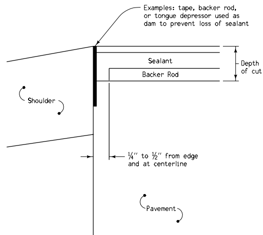
BACKER ROD PLACEMENT DETAIL
