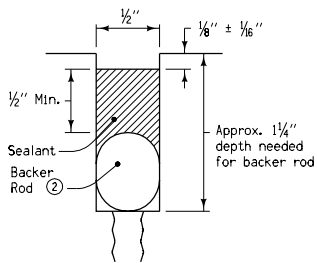
Note: Center 1/2" saw cut over the crack CLASS I CRACK RANDOM CRACK LESS THAN 1/2" IN WIDTH
