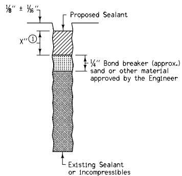
ALTERNATE BOND BREAKER FOR CLASS II CRACK CLASS IV JOINT CLASS V CRACK OR JOINT
