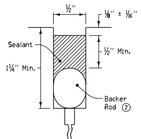
Note: Center 1/2" saw cut over existing joint CLASS III JOINT EXISTING JOINT LESS THAN 1/2" WIDE
