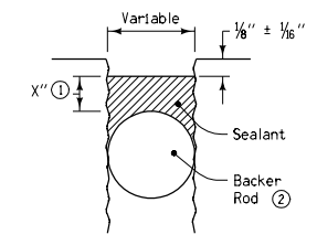
CLASS V CRACK OR JOINT EXISTING WIDTH 1 1/2"-3"
