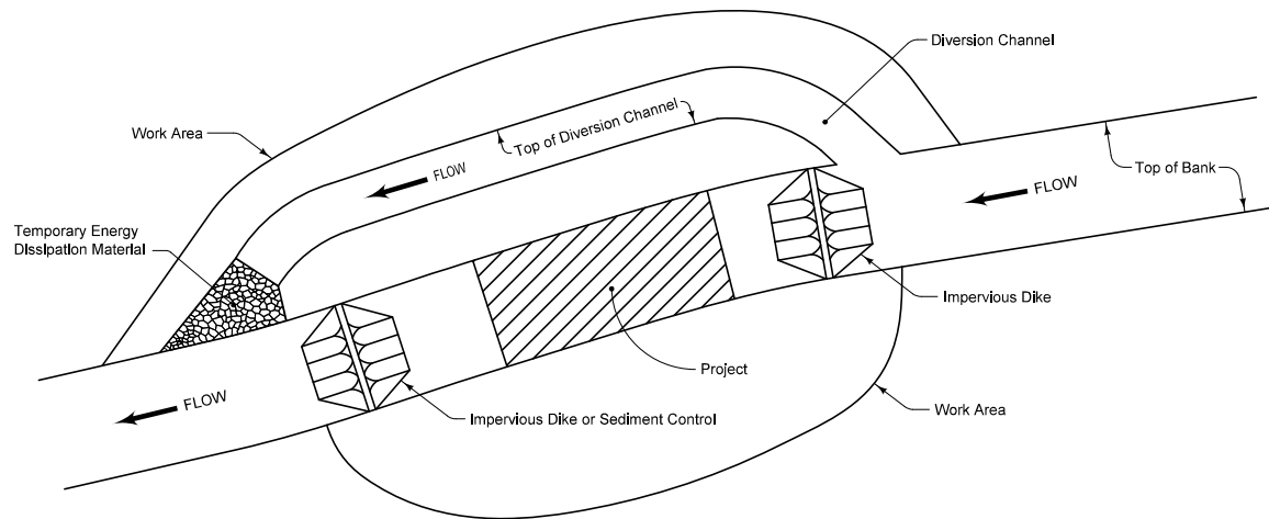
DIVERSION CHANNEL
