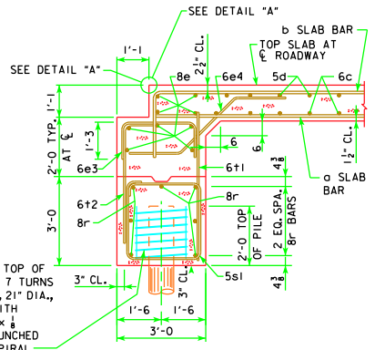
SECTION NORMAL TO ABUTMENT AT CL
