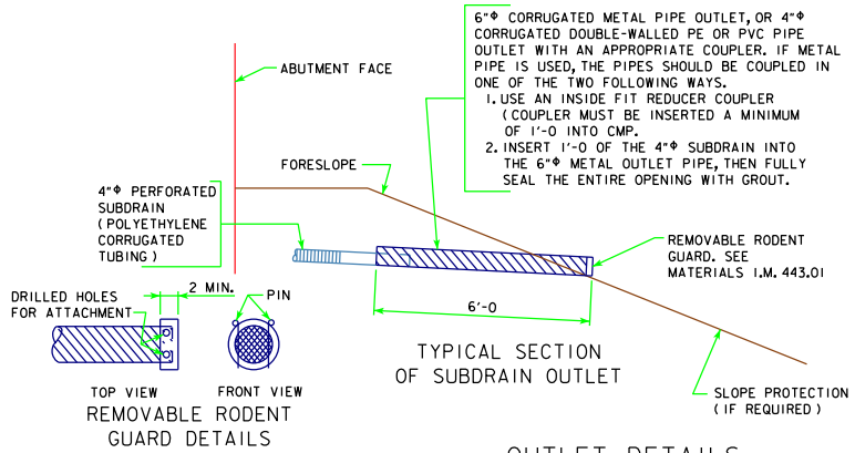
OUTLET DETAILS
