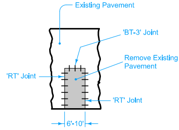
PARTIAL RAMP WIDTH PATCHES (NO EXISTING LONGITUDINAL JOINT)
