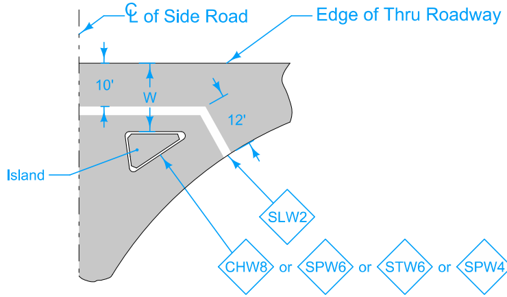
CASE 'C' ISLAND AND W ≥ 10 FT.
