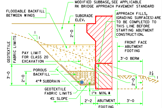
SECTION A-A BACKFILL DETAILS
