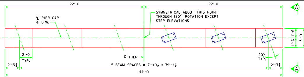
TYPICAL PLAN
