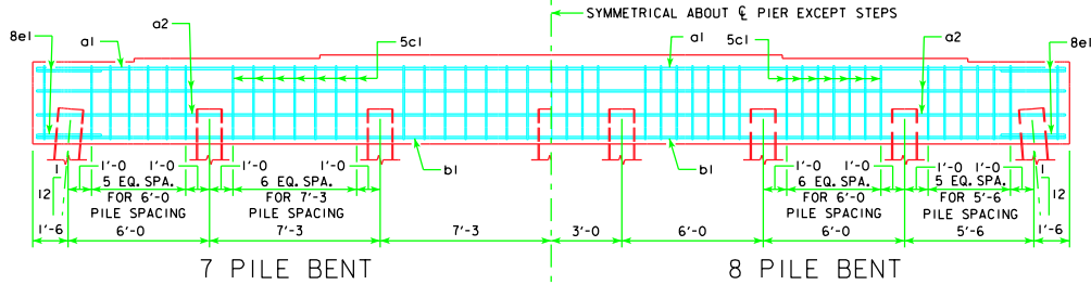
TYPICAL PLAN
