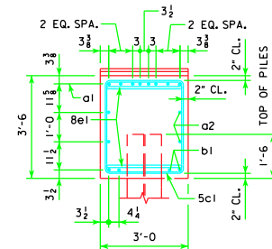
VIEW A-A FOR 7, 8, 9, 10, 11, 12 & 13 PILE BENTS
