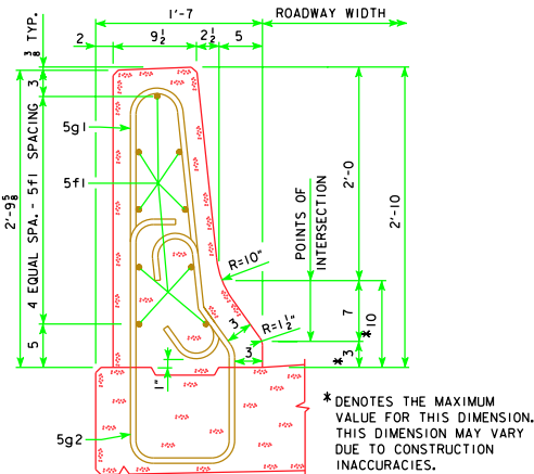
PART SECTION A-A
