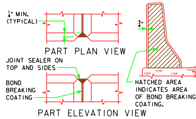
BARRIER RAIL JOINT DETAILS
