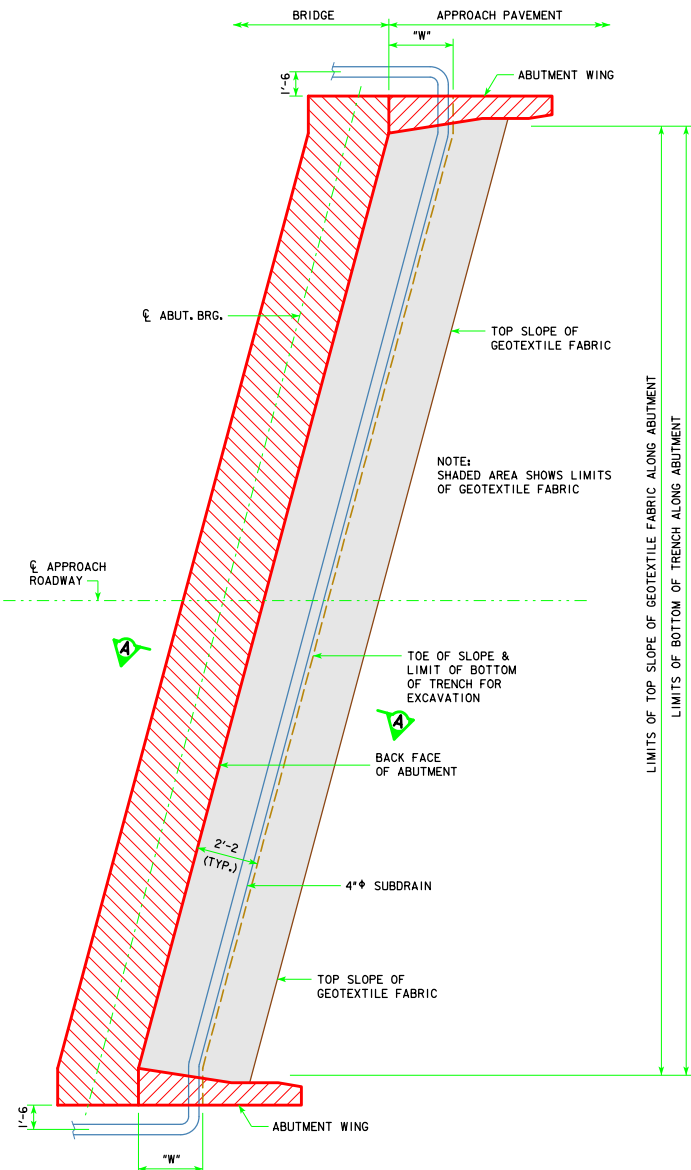
SKewed ABUTMENT PLAN WITHOUT WING EXTENSIONS (SKEWED LEFT AHEAD SHOWN, SKEWED RIGHT AHEAD SIMILIAR)
