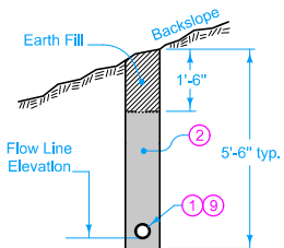
TYPE 11 INSTALLATION SECTION B-B Backslope
