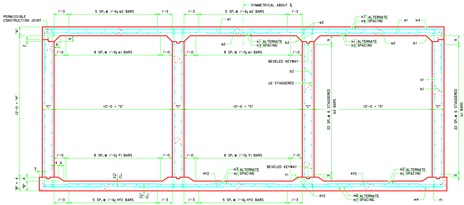
TRIPLE 10 x 12 BARREL SECTION
