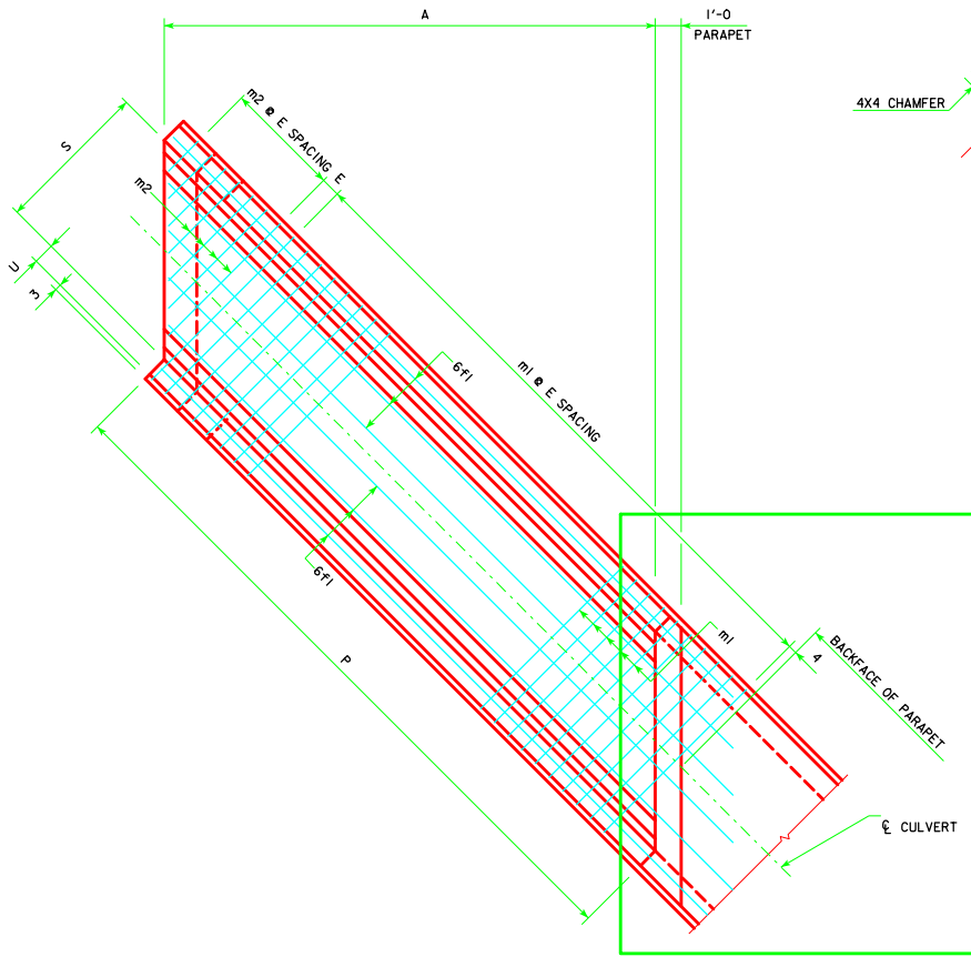
PLAN VIEW - TOP APRON REINFORCING
