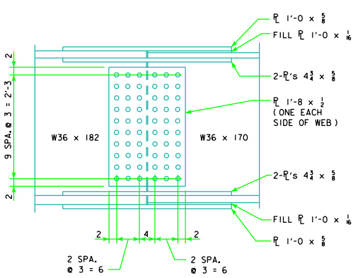
BOLTED SPLICE DETAILS
