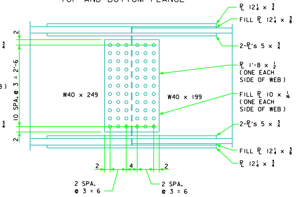
BOLTED SPLICE DETAILS
