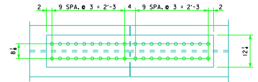
TOP AND BOTTOM FLANGE
