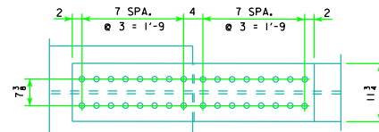
TOP AND BOTTOM FLANGE
