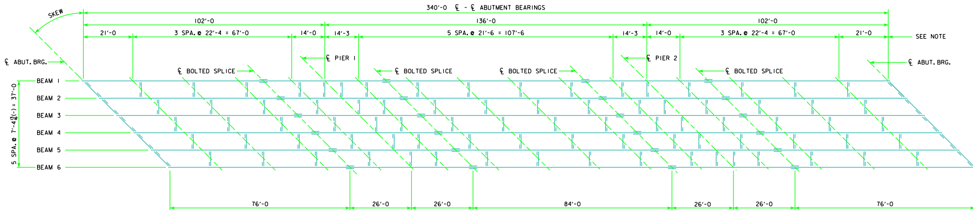
45° SKEWED FRAMING PLAN (R.A. SHOWN, L.A. SIMILAR)
