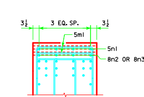
TYPICAL SECTION
