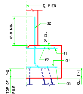
TYPICAL SECTION
