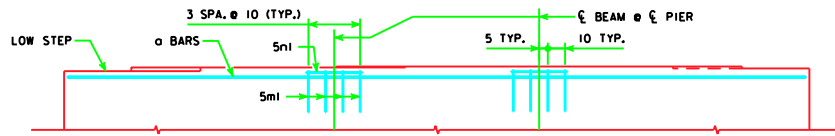
PART ELEVATION VIEW OF PIER CAP GRADE (G): G \leq 0.6\%
