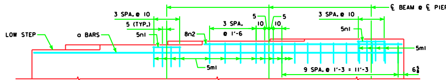
PART ELEVATION VIEW OF PIER CAP GRADE (G): 4.0\% < G \leq 5.0\%
