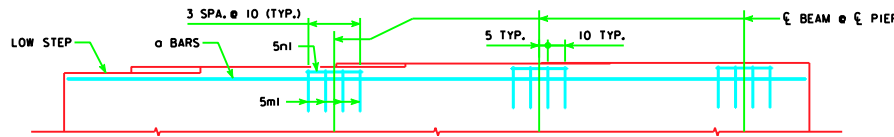
PART ELEVATION VIEW OF PIER CAP GRADE (G): 0.6\% < G \leq 2.3\%
