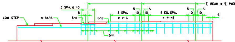
PART ELEVATION VIEW OF PIER CAP GRADE (G): 2.3\% < G \leq 4.0\%
