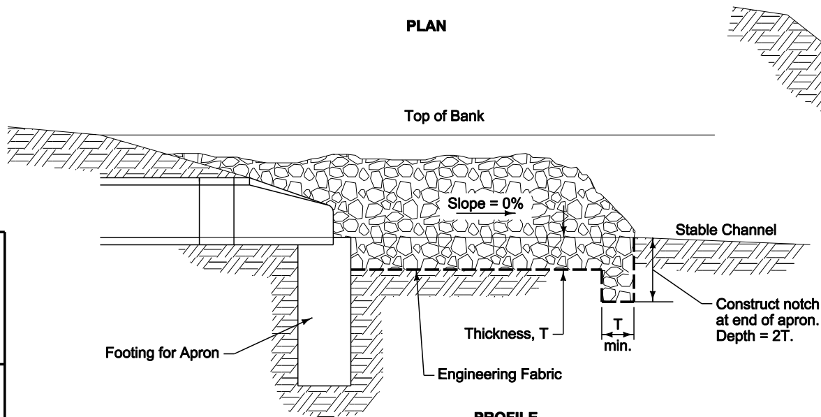
PROFILE Section A-A
