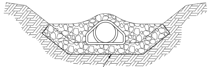
CROSS-SECTION
