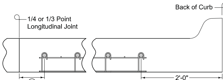
PLACEMENT LIMITS (Curb and Gutter - 1/4 or 1/3 Point Jointing)
