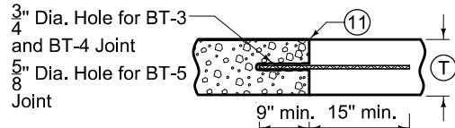
ABUTTING PAVEMENT JOINT - RIGID TIE (Drilled)
