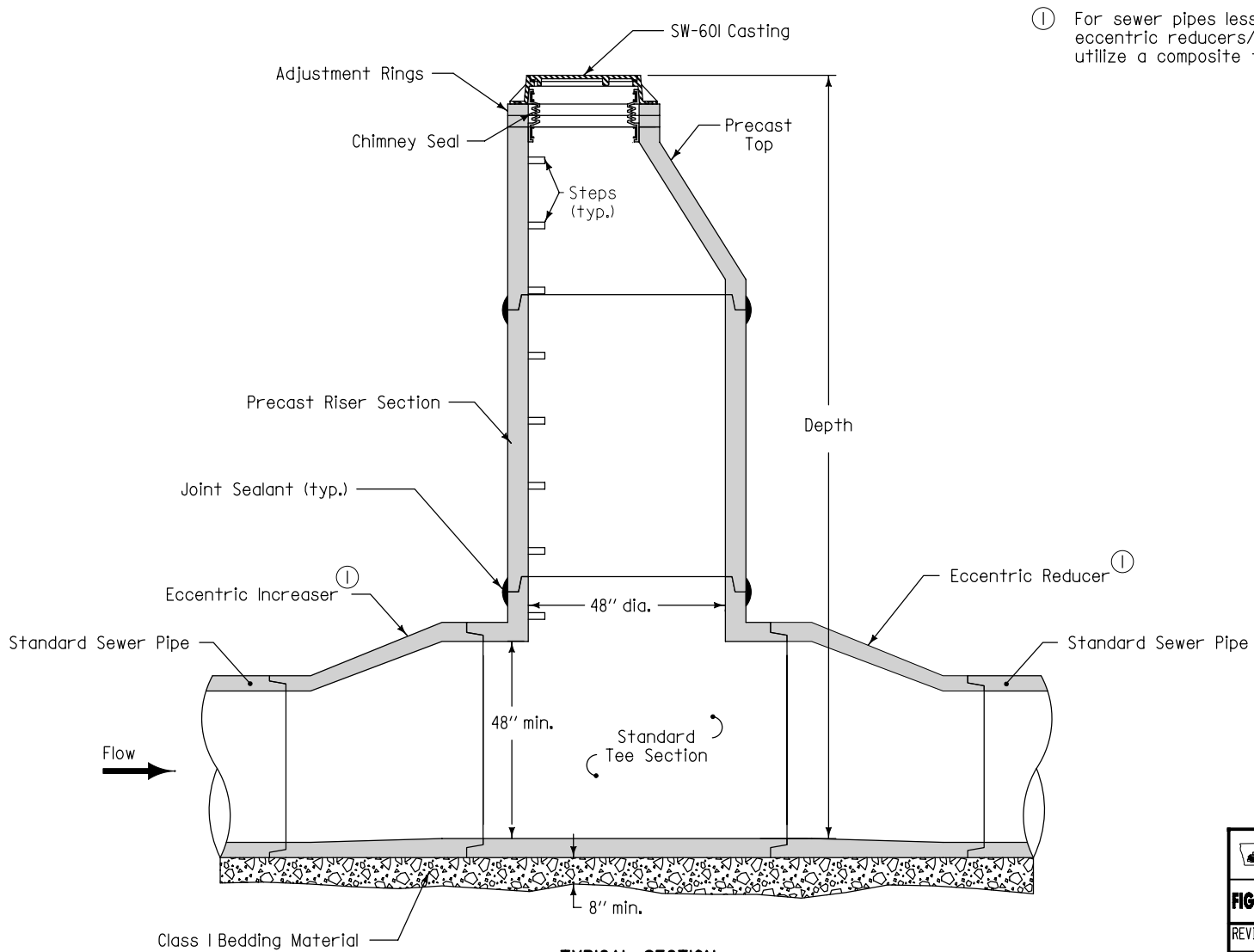
TYPICAL SECTION STANDARD TEE ①
